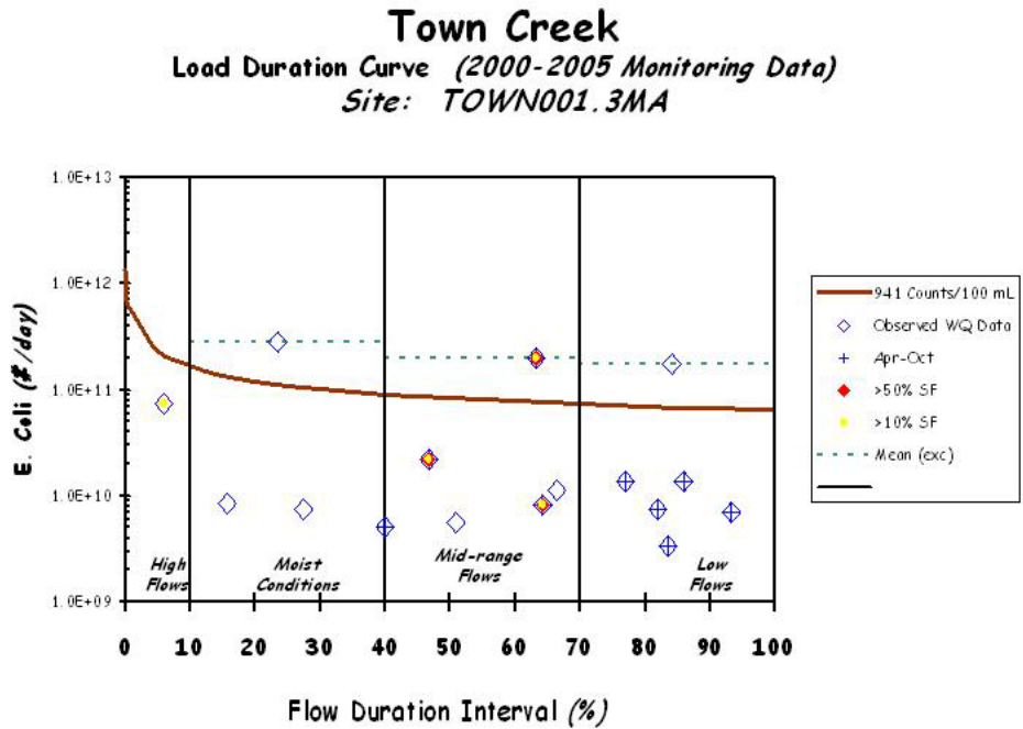
Figure E-4. E. Coli Load Duration Curve for Town Creek at Mile 1.3
