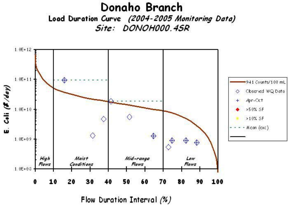
Figure E-3. E. Coli Load Duration Curve for Donaho Branch
